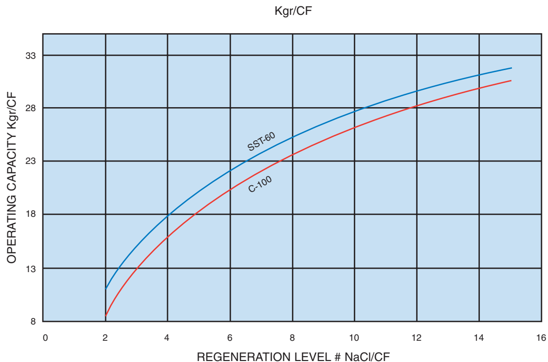
Fig. 5 OPERATING CAPACITY
