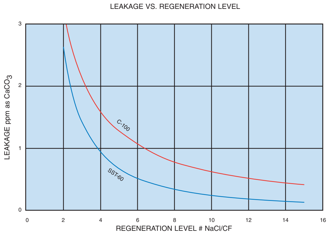
Fig. 6 LEAKAGE VS. REGENERATION LEVEL
