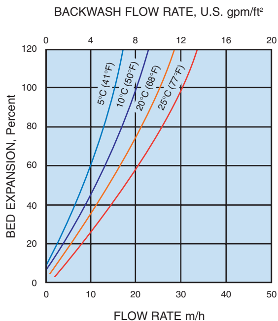
Fig. 4 BACKWASH EXPANSION
